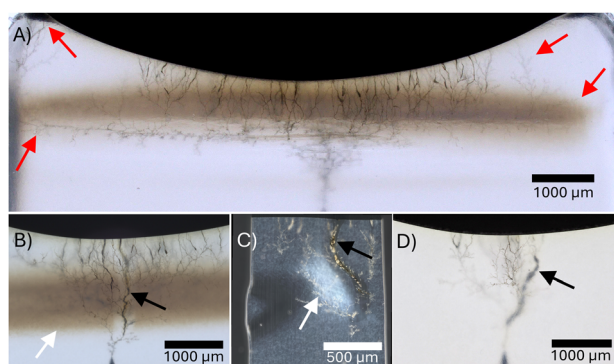
Fig. 8 Optical images of electrical treeing until breakdown in samples with (A, B and C) and without (D) stress whitening; (A) extreme branching without reaching breakdown, front view (PP SW 5); (B) breakdown in the stress-whitened region, front view (PP SW 4); (C) breakdown in the stress-whitened region, side view of a 150 \mu\text{m} microtomy slice (PP SW 4); (D) breakdown in an unstressed sample (PP 3). Arrows indicate the breakdown channel (black), stress-whitened area (white) and branching at extremities (red).
