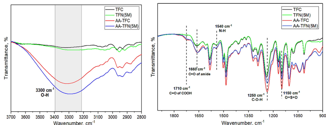
Fig. 3. ATR-FTIR spectra of different composite membranes, (a) 3700 to 2800 cm -1 and (b) 1900 to 900 cm -1 .
