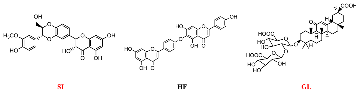
Fig. 1. Structures of SI, HF and GL.
